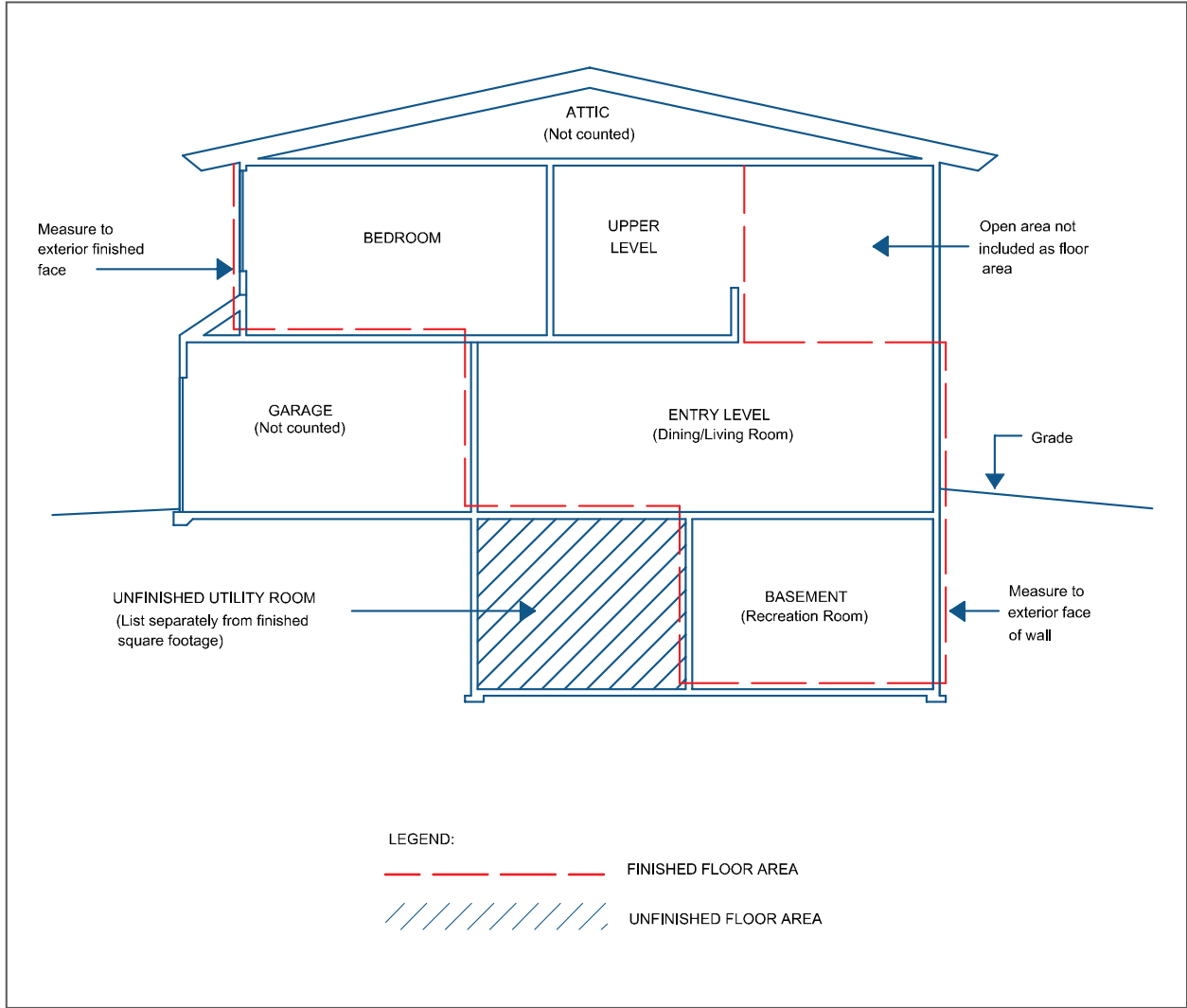
FIGURE 4. Building Section
